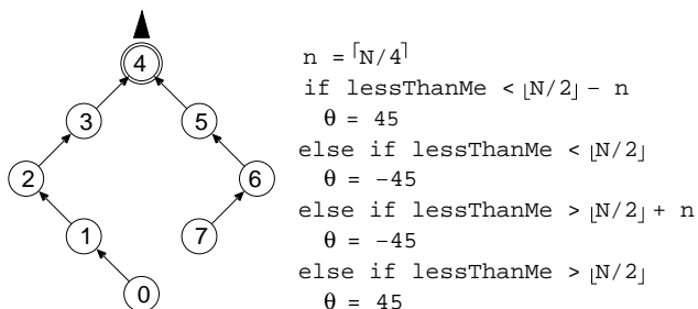
Fig. 2. Calculating the friendship angle in a diamond with 8 robots. The diamond is a centered formation, so the robot with the median ID ( lessThanMe = \lfloor N/2 \rfloor ) is the conductor. Arrows indicate angle to friend, filled triangle shows formation heading.
